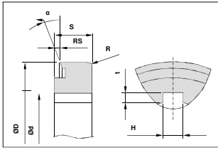
type NN with groove
