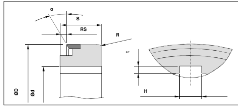
type NN-TCT with groove
