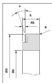
type NN without groove
