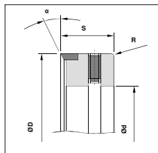
type NS-TCT with screw fixing
