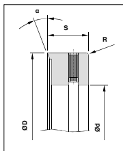
type NS with screw fixing
